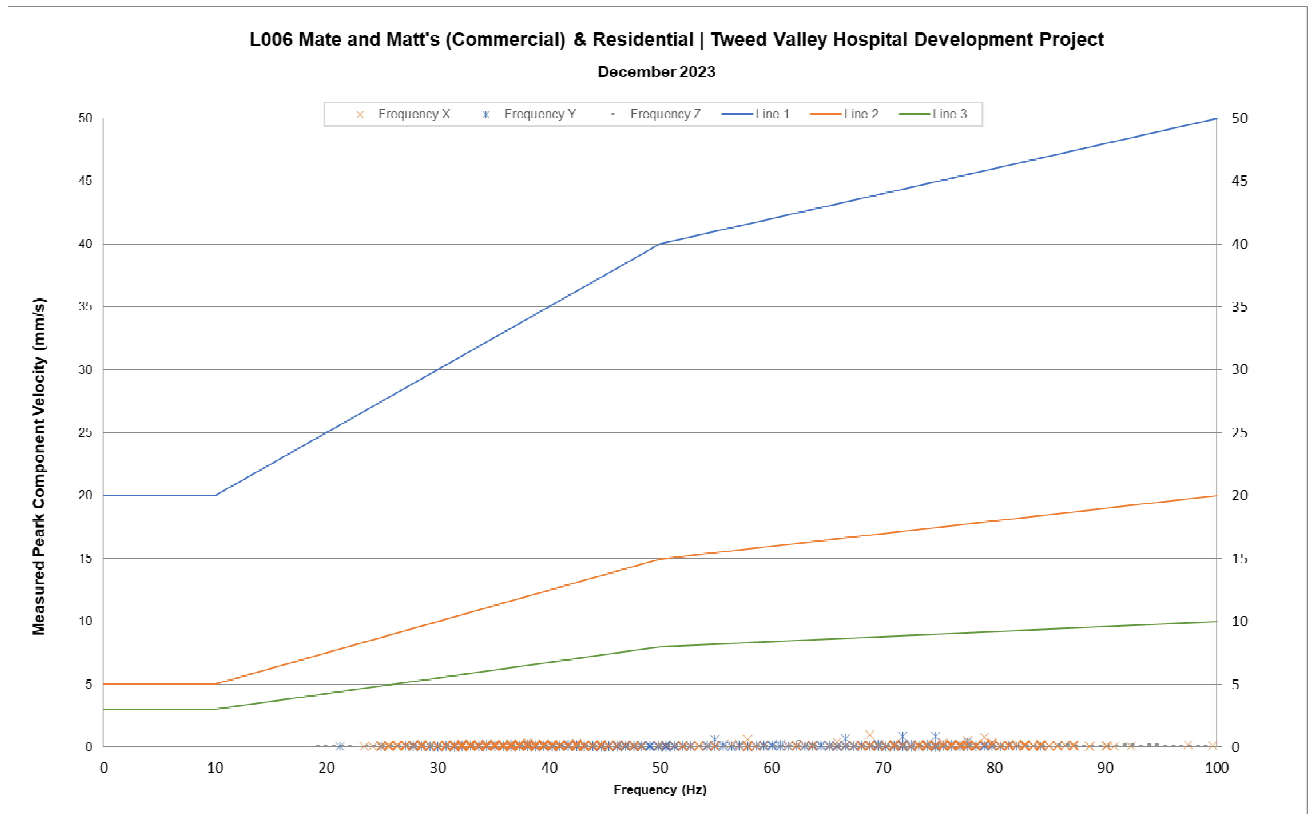
Figure 3 Frequency over Velocity (Logger 006 – Residential/Commercial)
