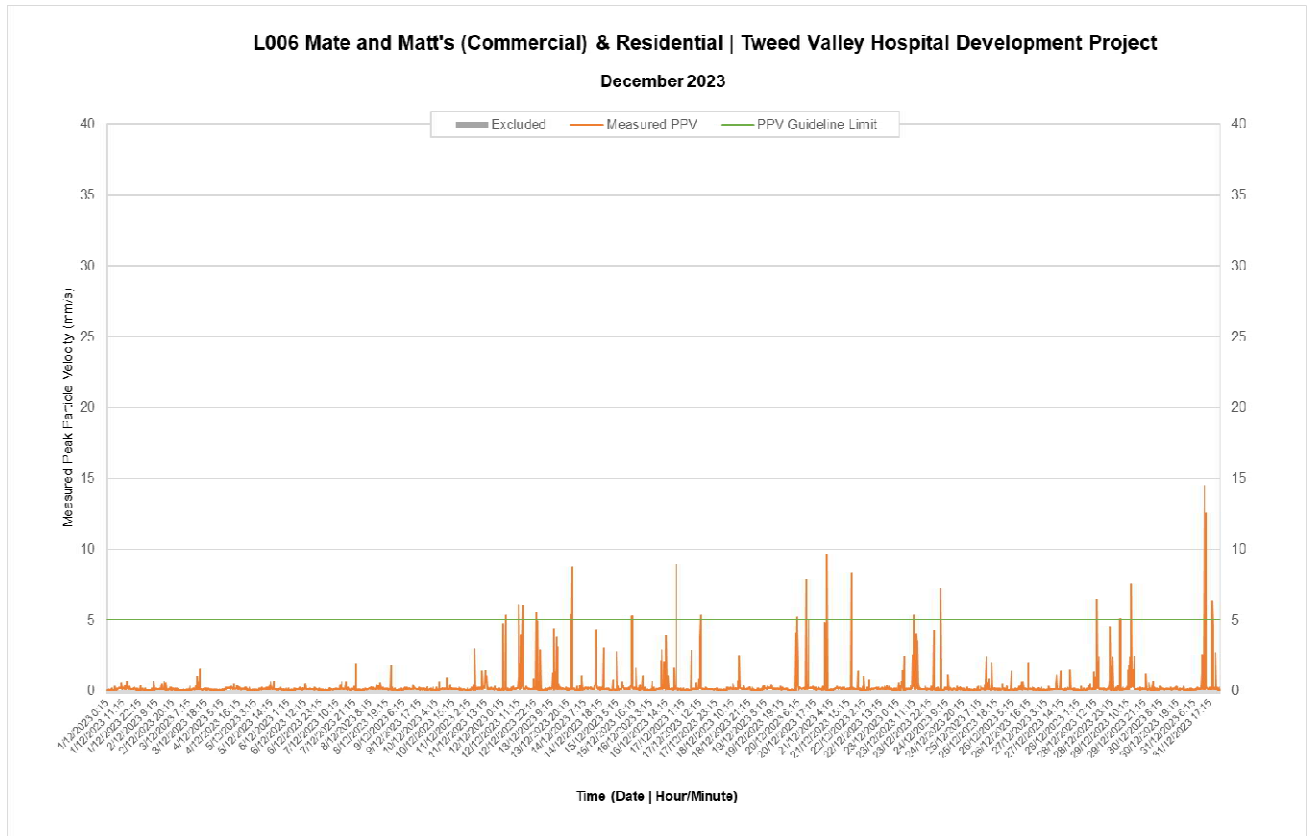
Figure 2 Velocity over time (Logger 006 – Residential/Commercial)
