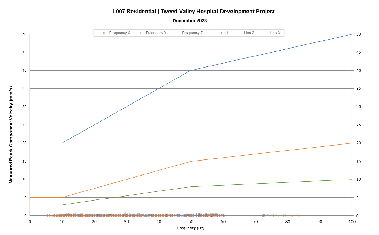
Figure 5 Frequency over Velocity (Logger 007 – Residential)
