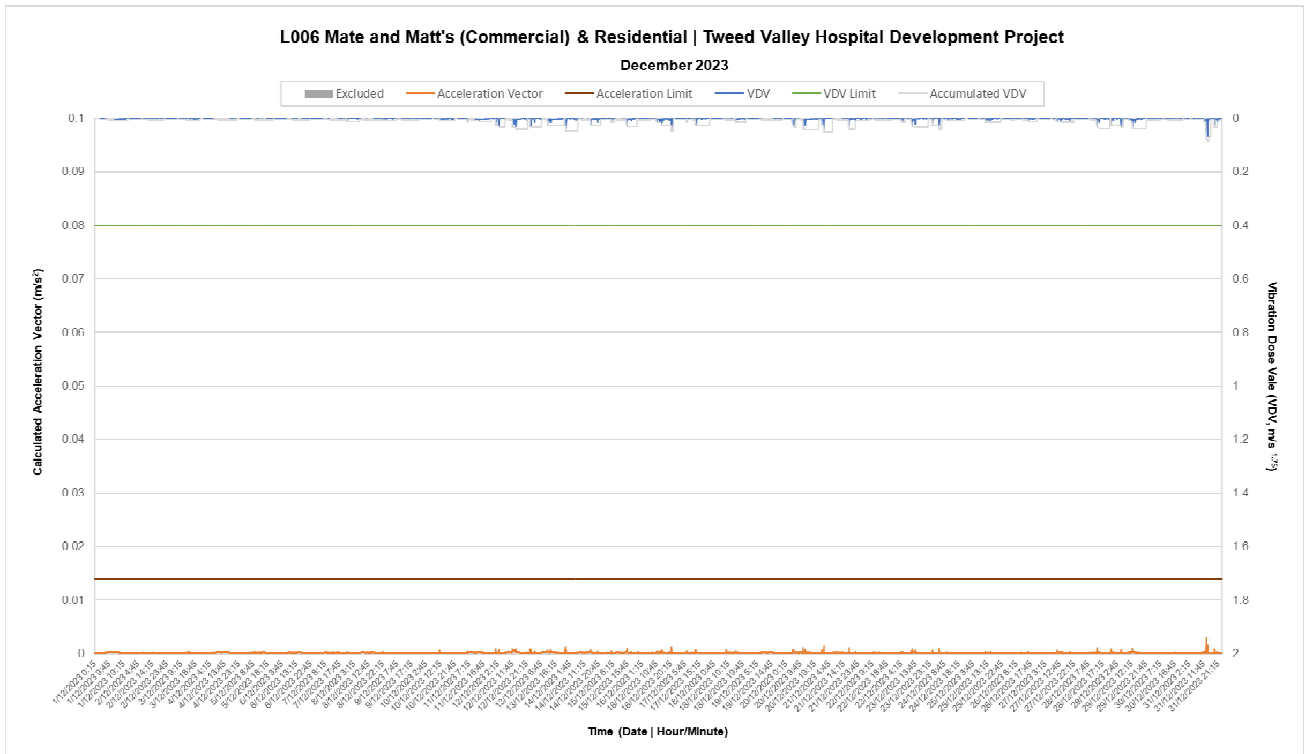
Figure 6 Acceleration and Vibration Dose Value over time (Logger 006 – Residential/Commercial)
